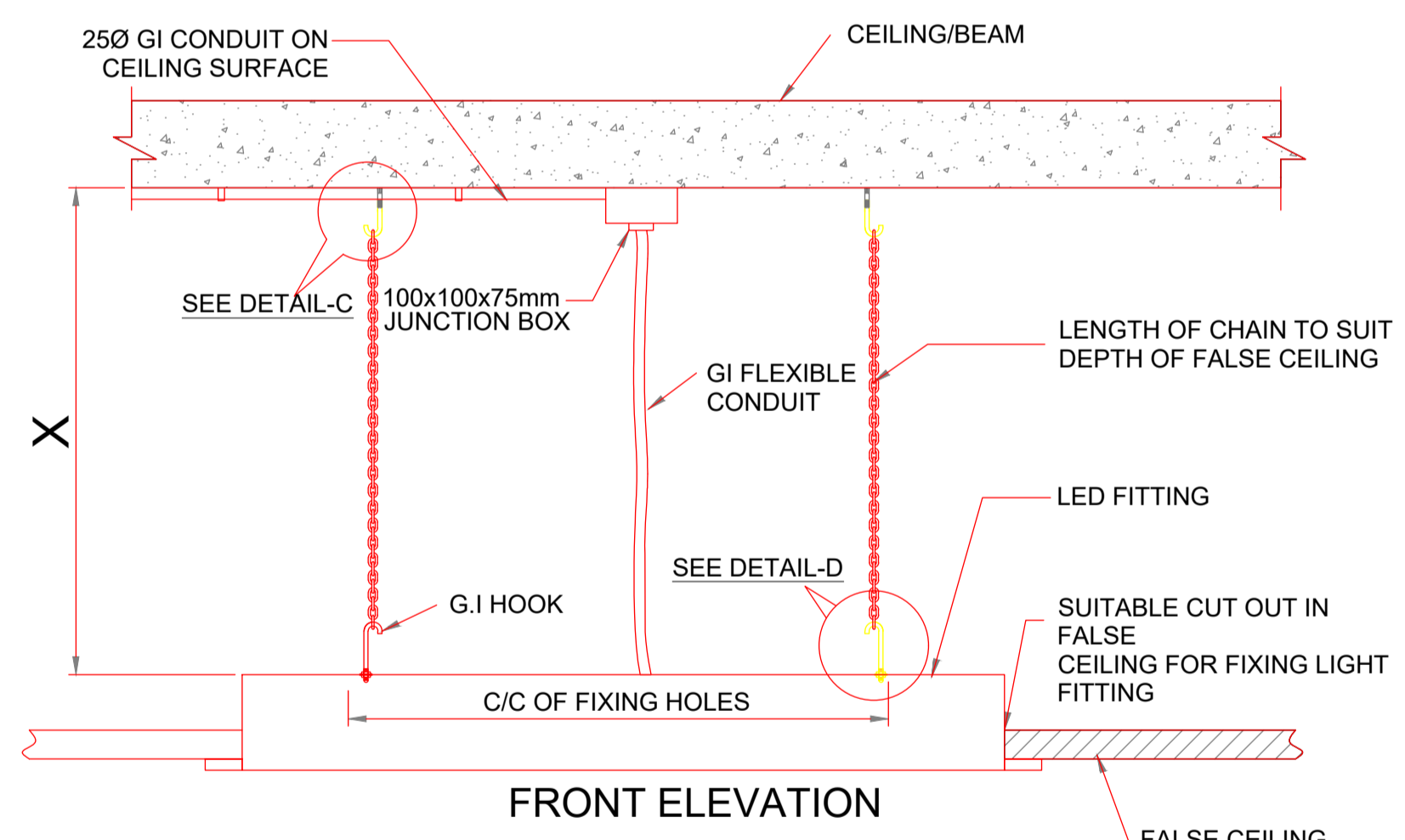
LDB MOUNTING ARRANGEMENT
