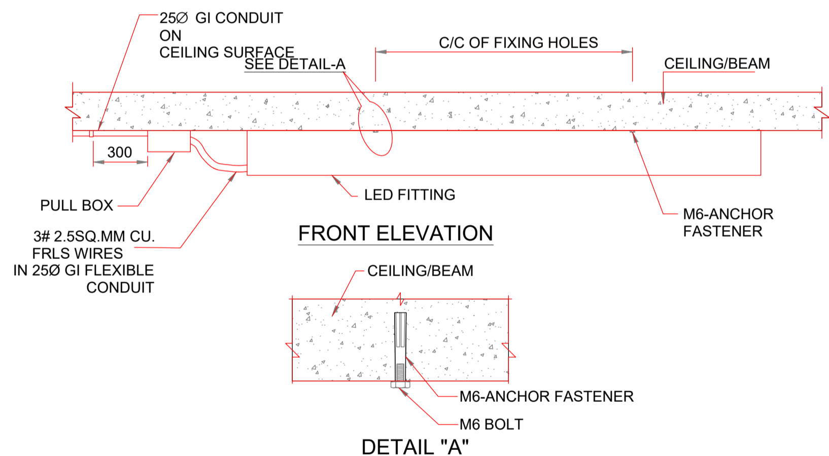
SURFACE MOUNTING FITTING ARRANGEMENT
