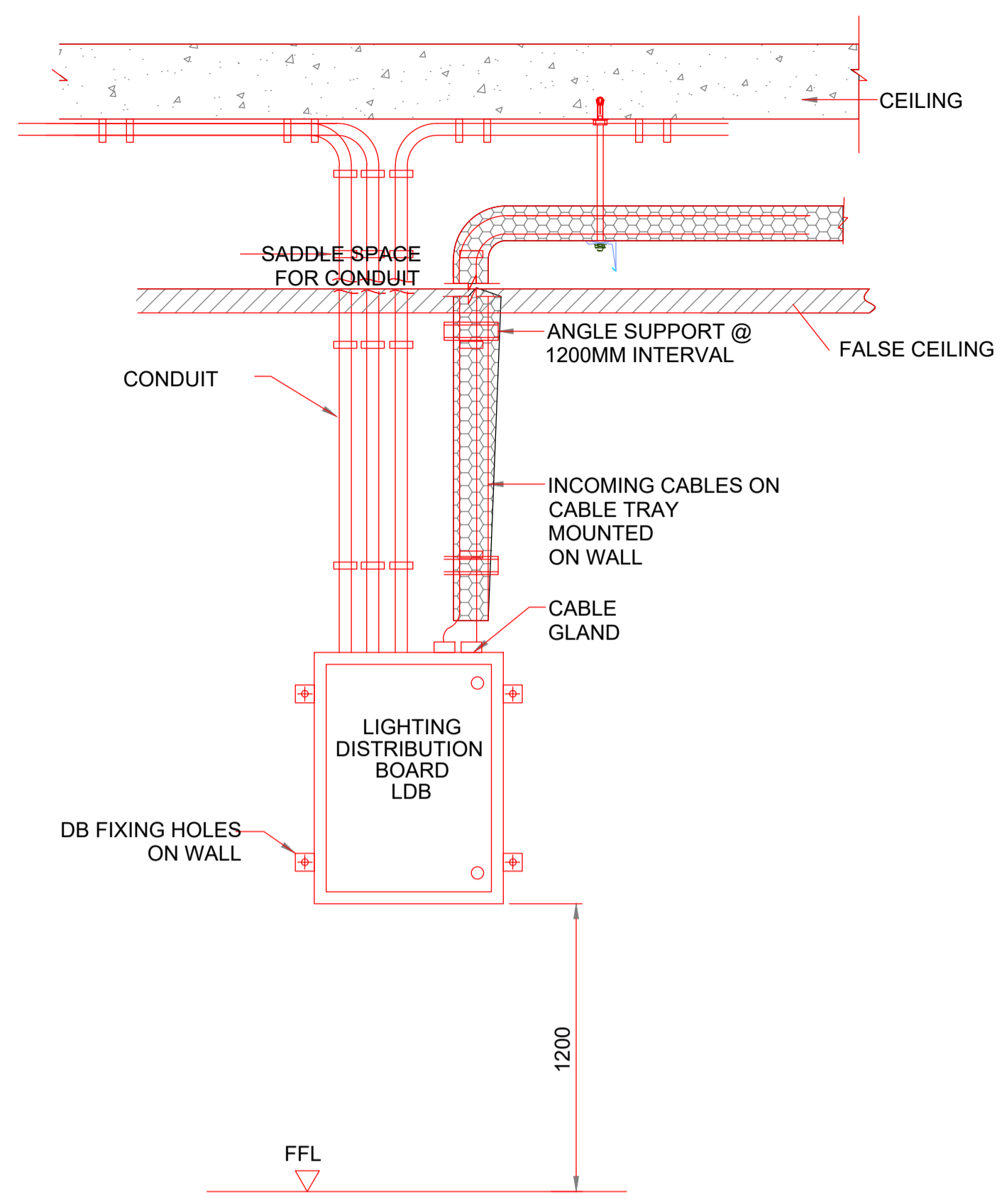
LDB MOUNTING ARRANGEMENT
