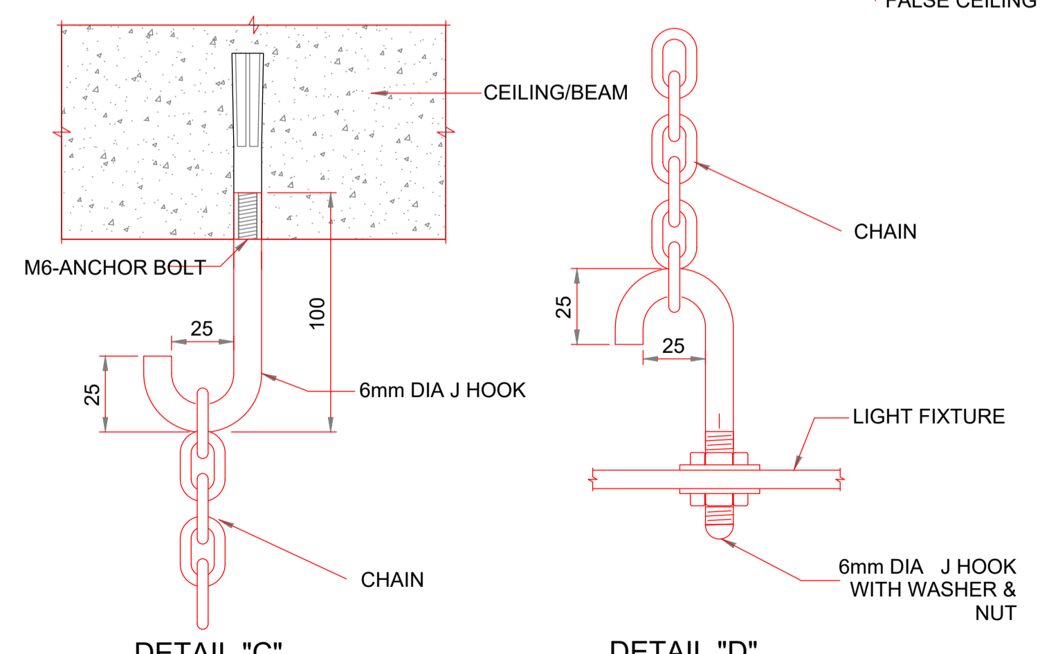
DETAIL "C" CEILING SUSPENDED FITTING ARRANGEMENT WITH CHAIN & HOOK
